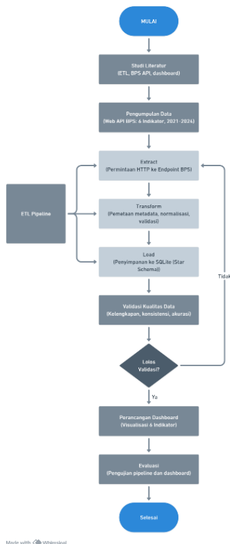
GAMBAR III.1 Alur Penelitian ETL Pipeline & Dashboard Analitik
